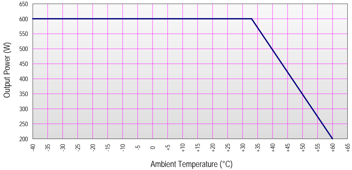
INMSW600B-24/115 Power Derating Curve
